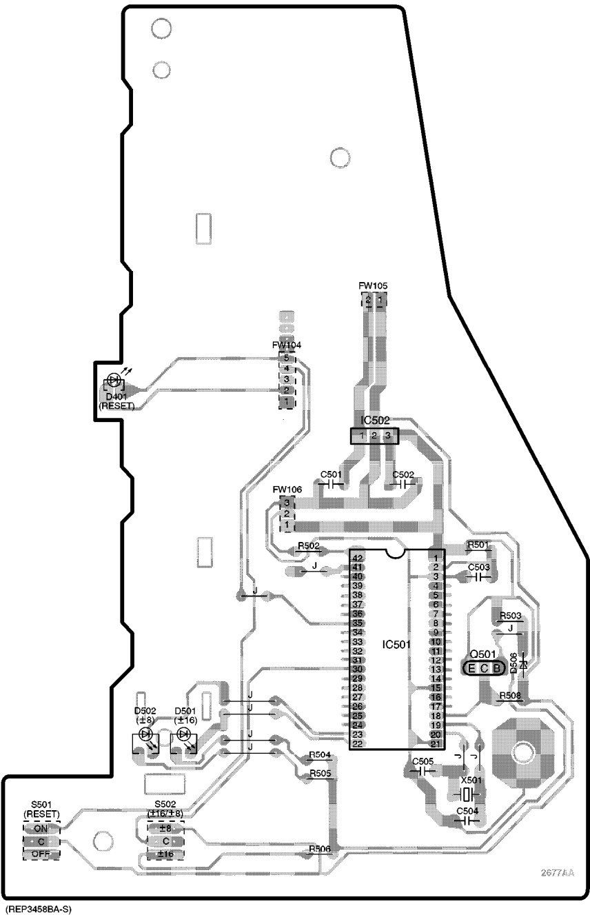
H PITCH CONTROL(1) P.C.B.
