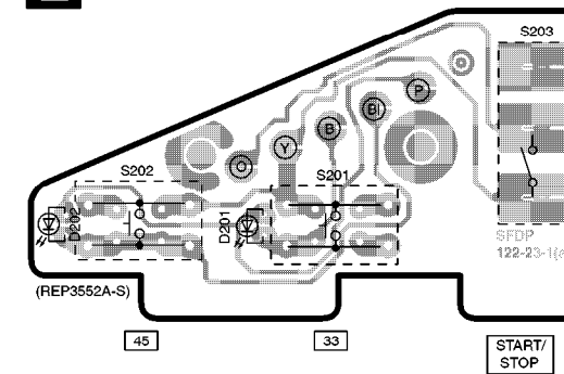
E SPEED SELECTOR P.C.B.
