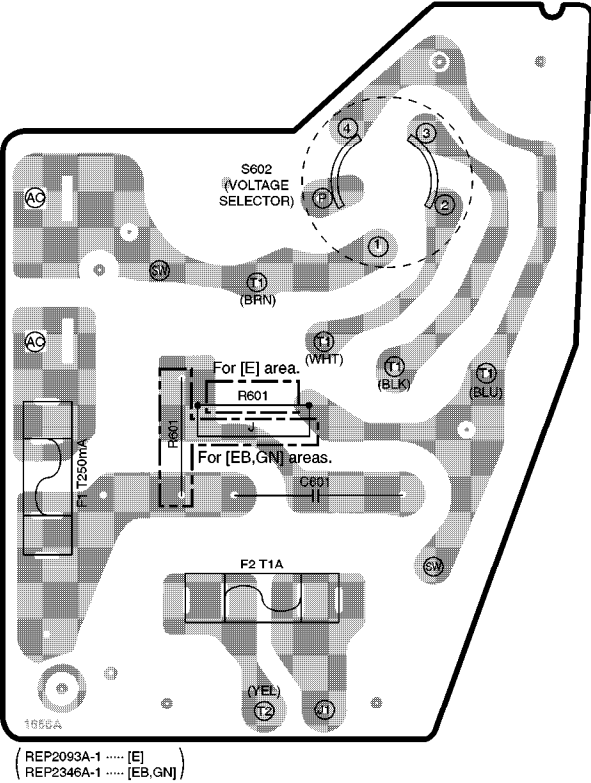
B POWER SUPPLY P.C.B. For [E,EB,GN] areas.
