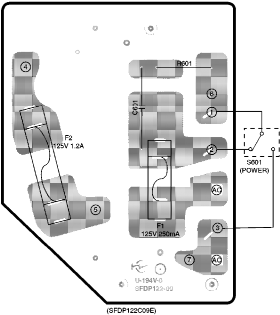
B POWER SUPPLY P.C.B. For [PP] area.
