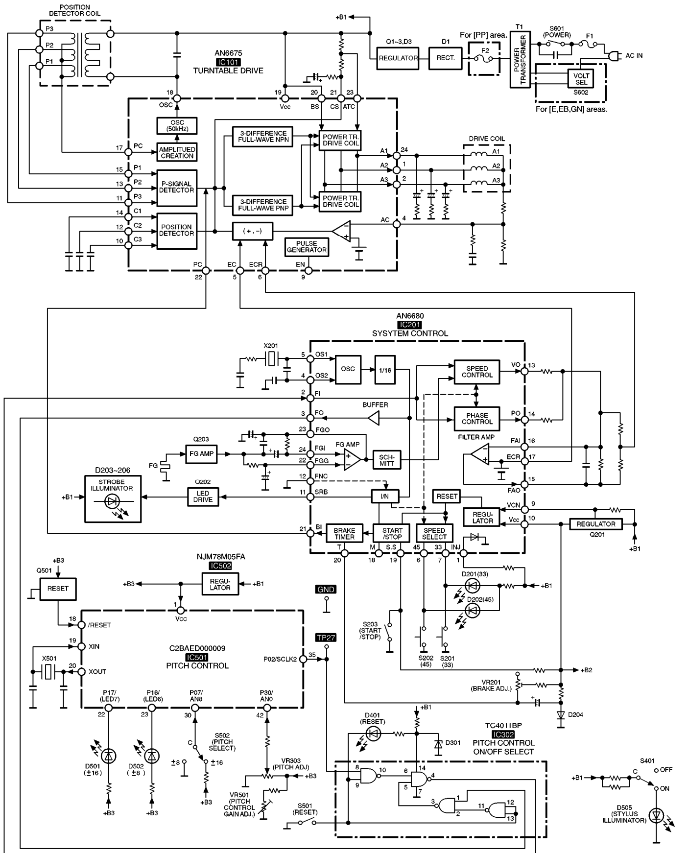
SL-1210M5G(P,P,E,B,G,N) BLOCK DIAGRAM
