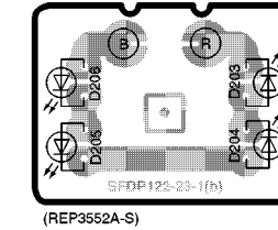
D STROBE ILLUMINATOR P.C.B.
