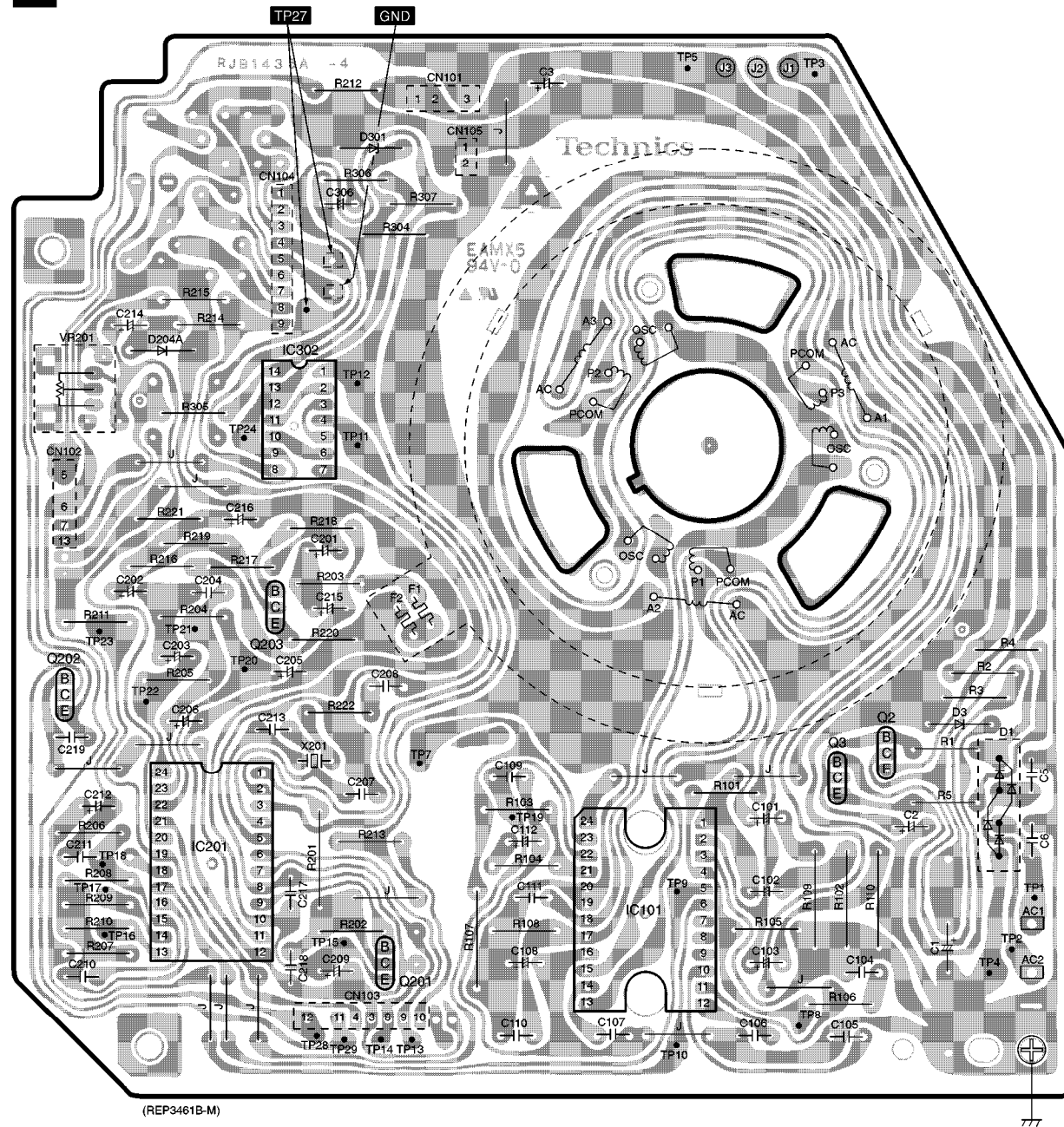
A DRIVE CONTROL P.C.B.
